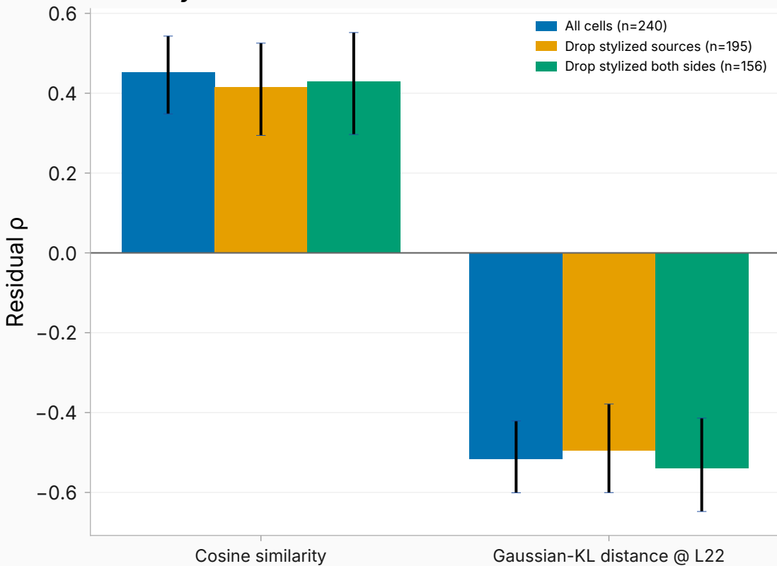
Ordinary cross-context
