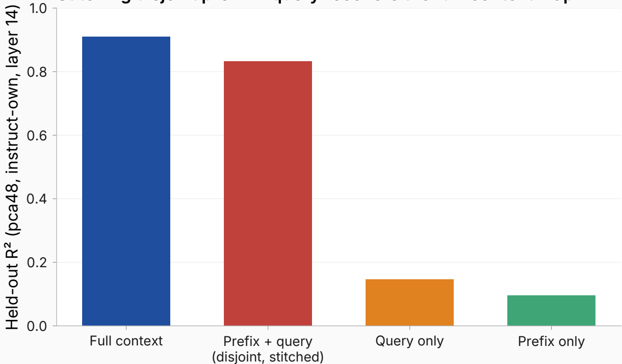
Stitching disjoint prefix + query recovers the full-context map
