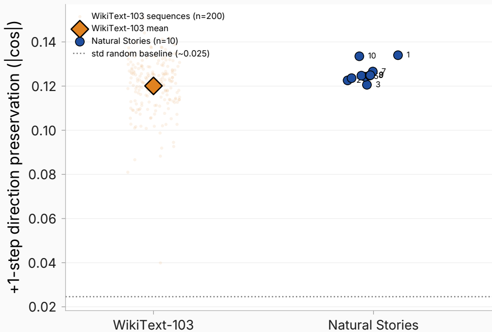
mid-band (layer 13)
