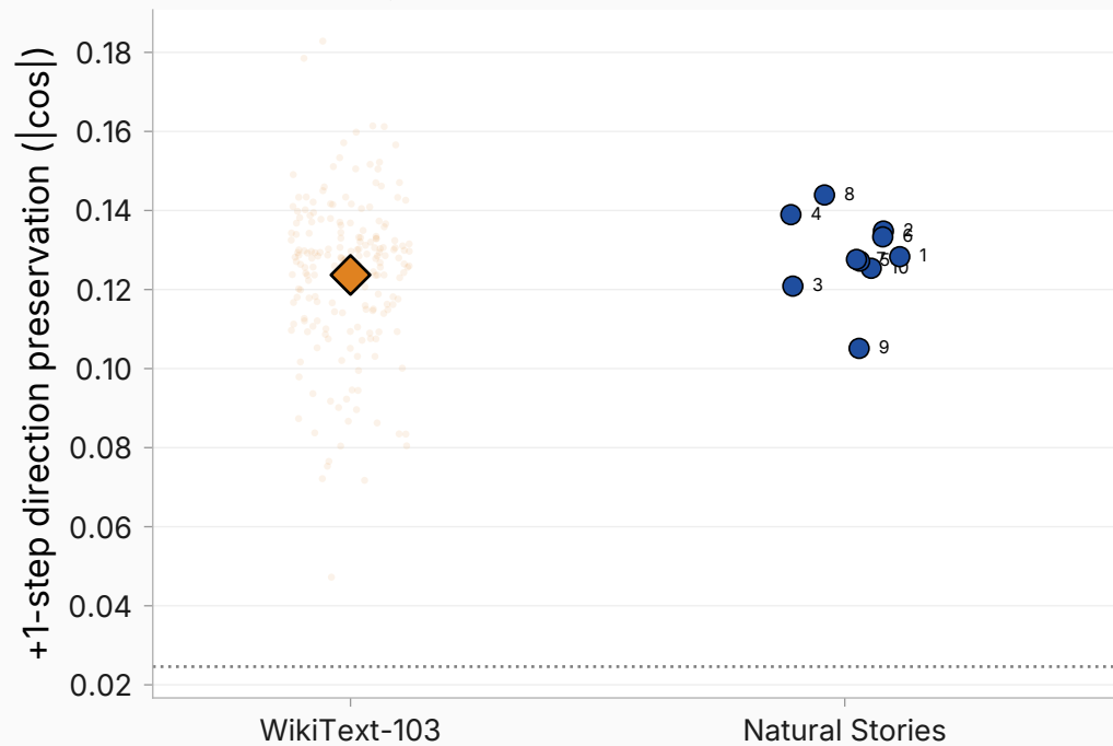
late-band (layer 27)
