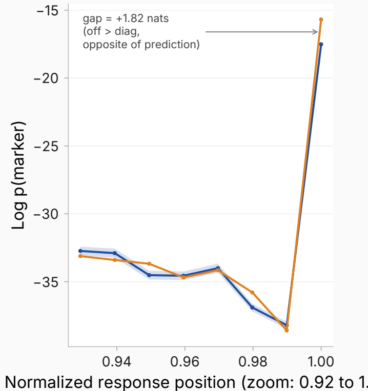
Zoom: off-diagonal endpoint higher than diagonal
