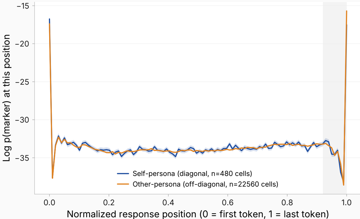
Full trajectory (boundary spikes are np.interp artifacts at varying lengths)
