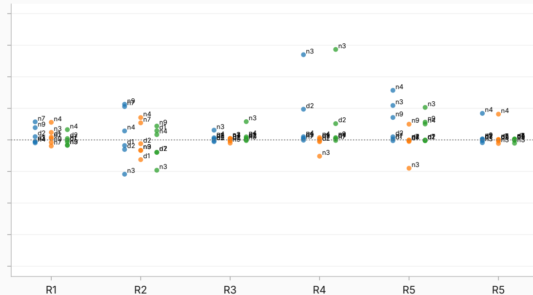
erase — prefix-end
