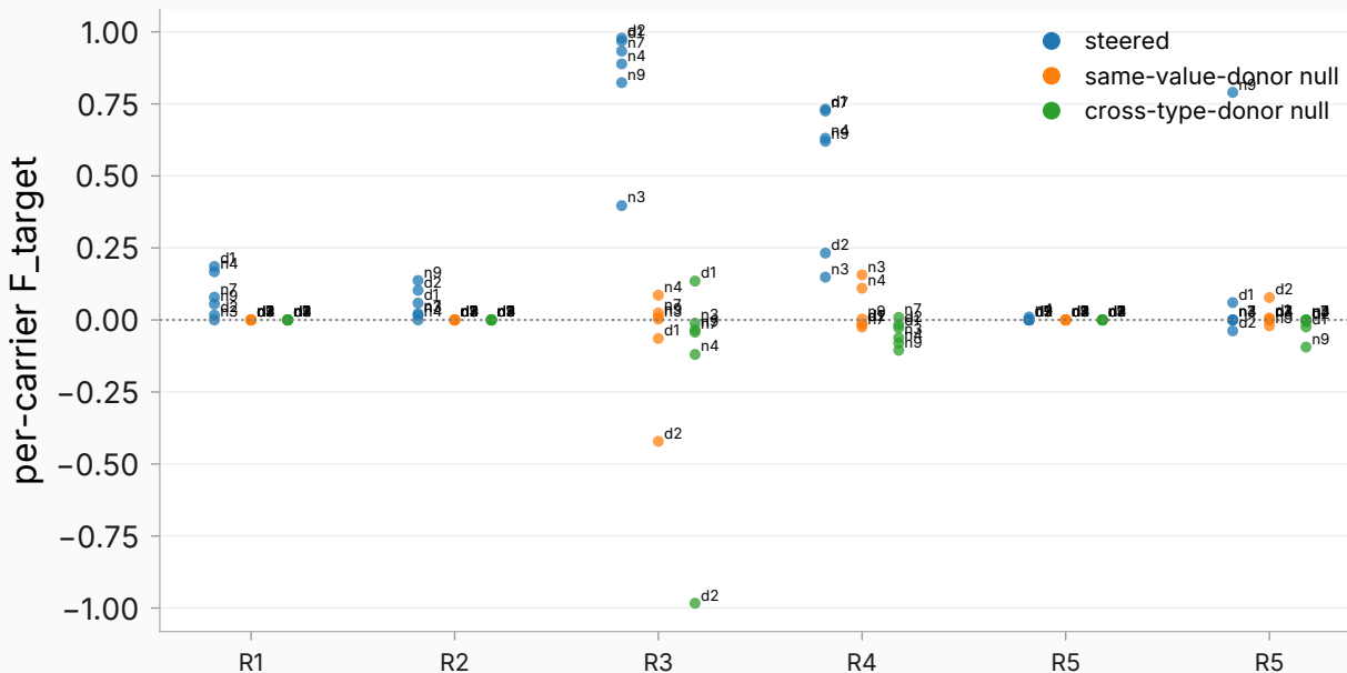
install — prefix-end
