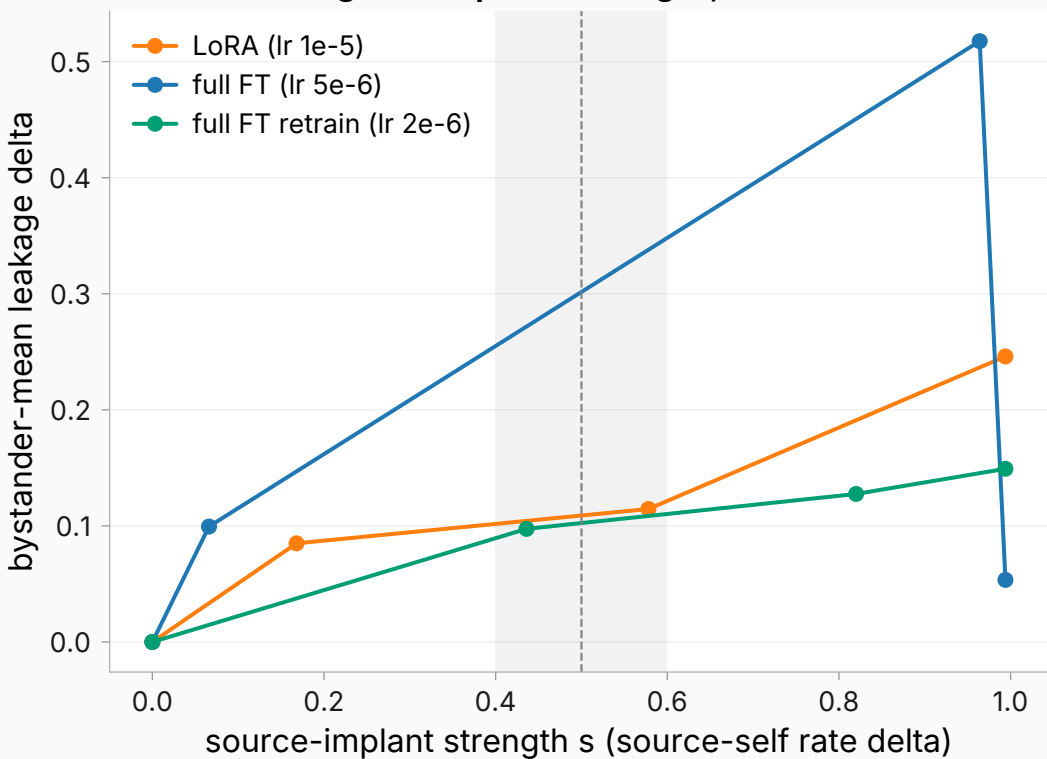
refusal: leakage vs implant strength, with the lr 2e-6 full-FT retrain
