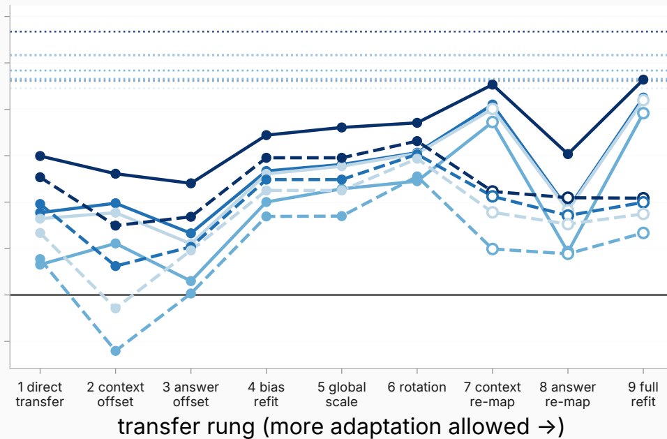
Qwen2.5-7B-Instruct
