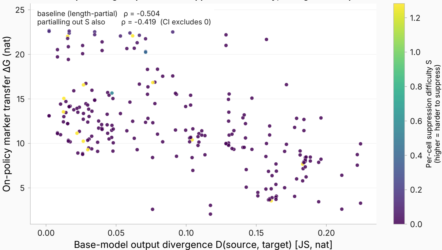
Even after partialling out per-source suppression difficulty, divergence still predicts transfer
