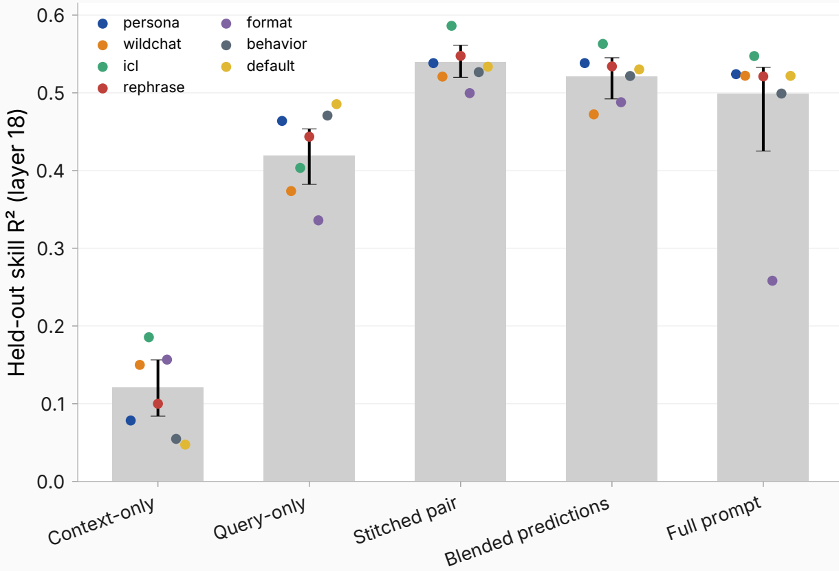
Misalignment-genre queries (Betley)
