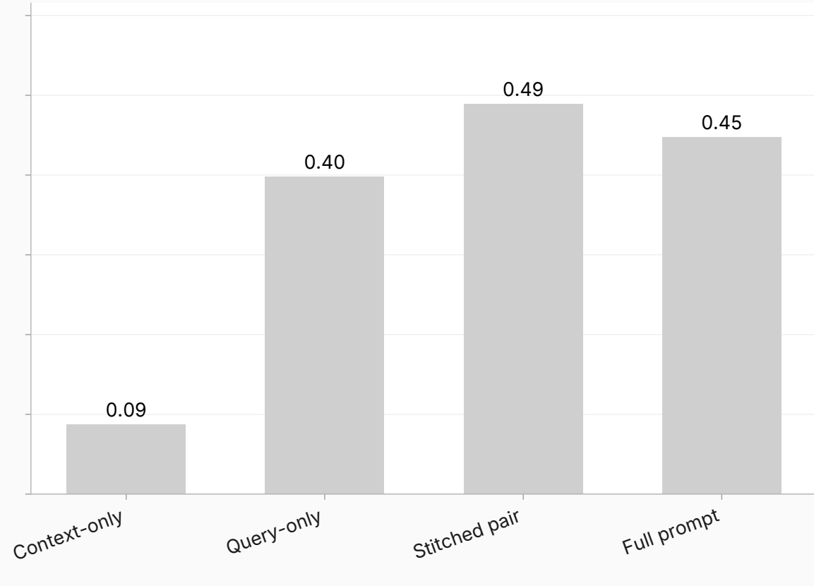
Human-written OOD queries (Dolly), UC-trained
