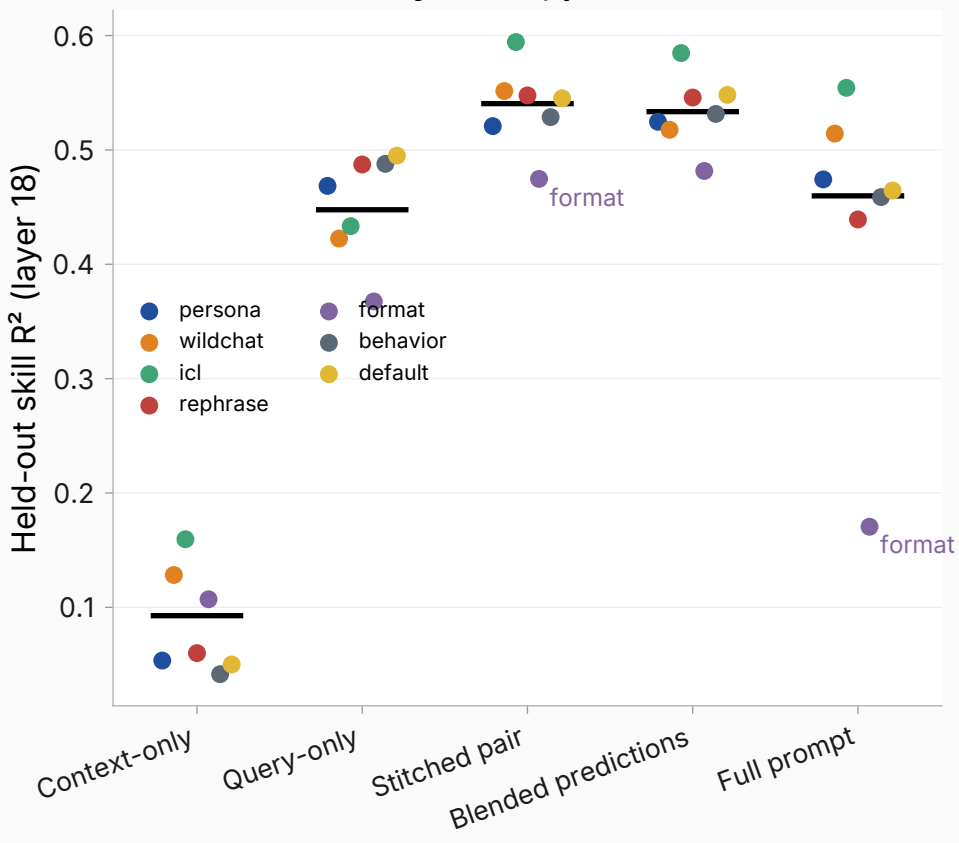
Per held-out family (dots); pooled (bar)
