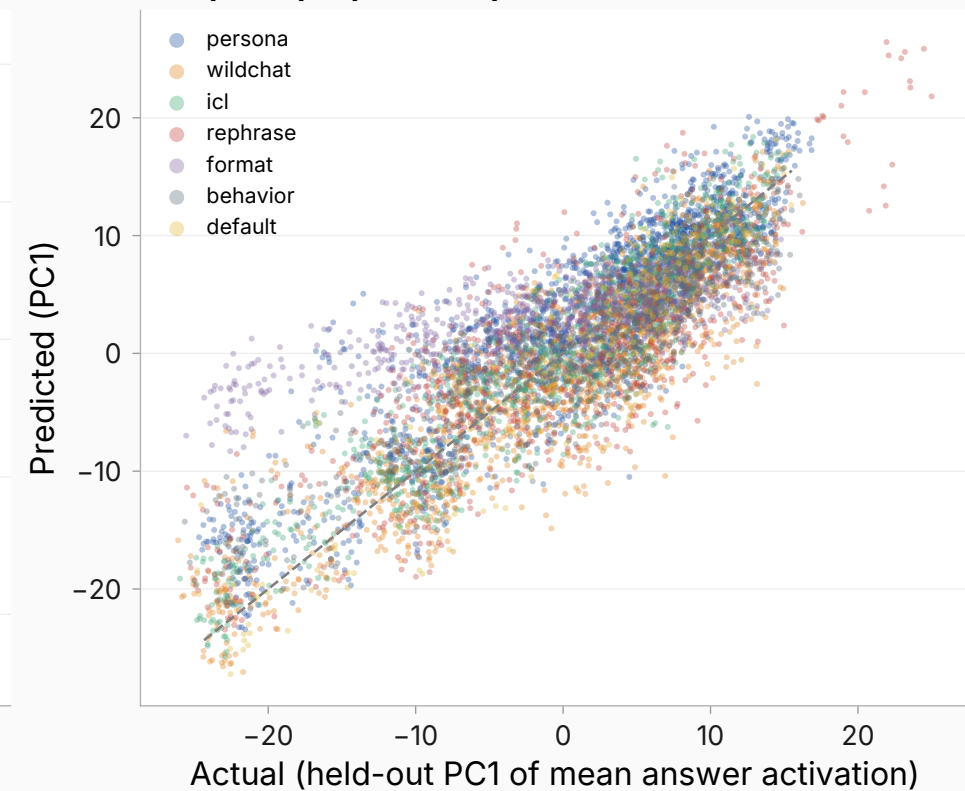
Full prompt: per-cell predictions (n=7200)
