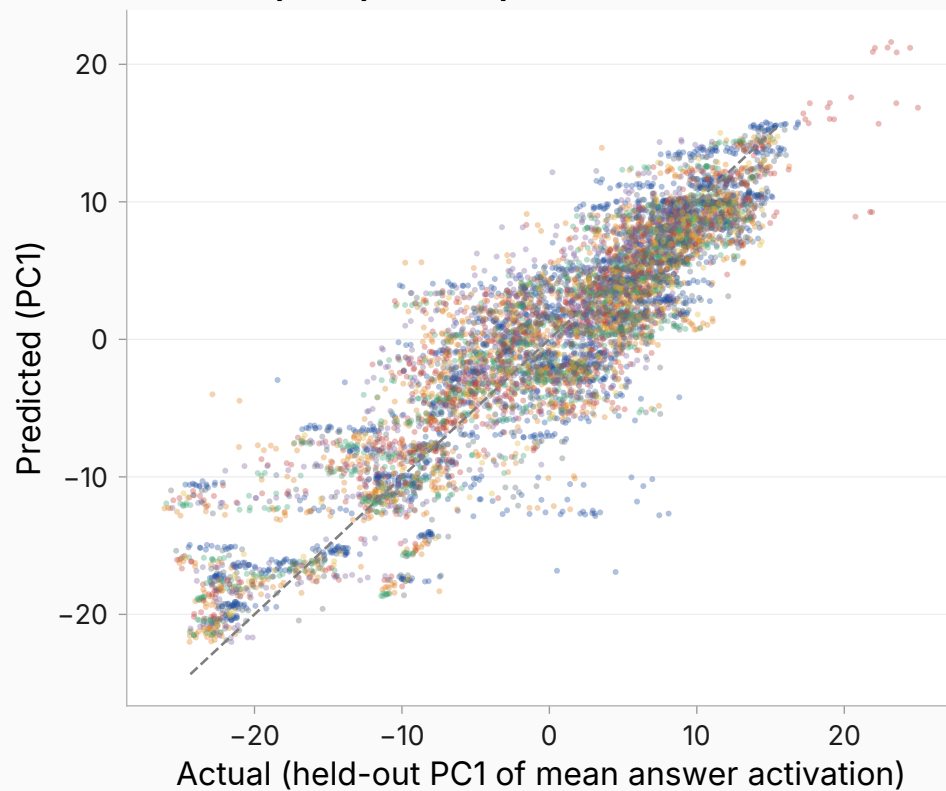
Stitched pair: per-cell predictions (n=7200)
