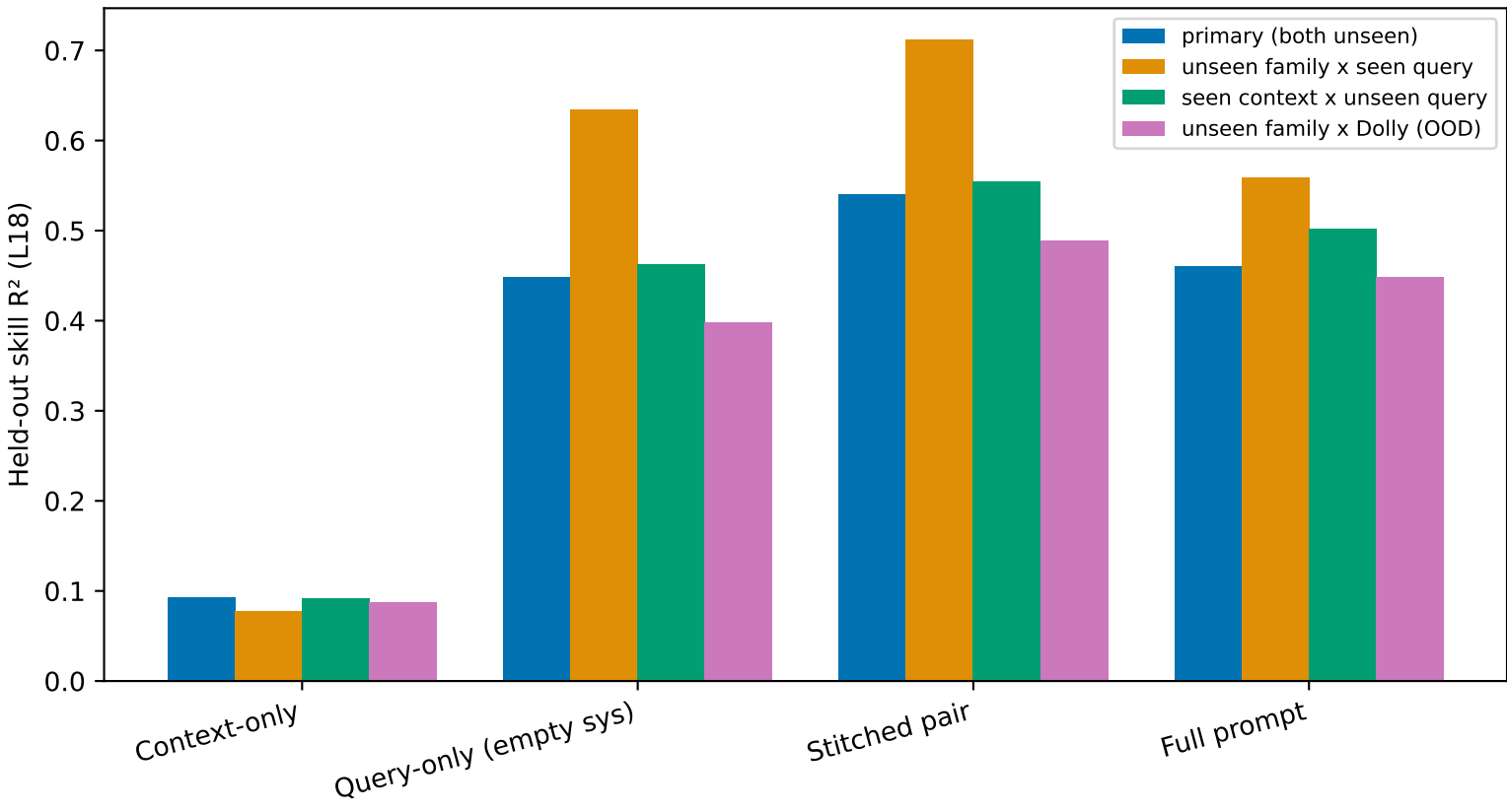
Fold regimes — uc
