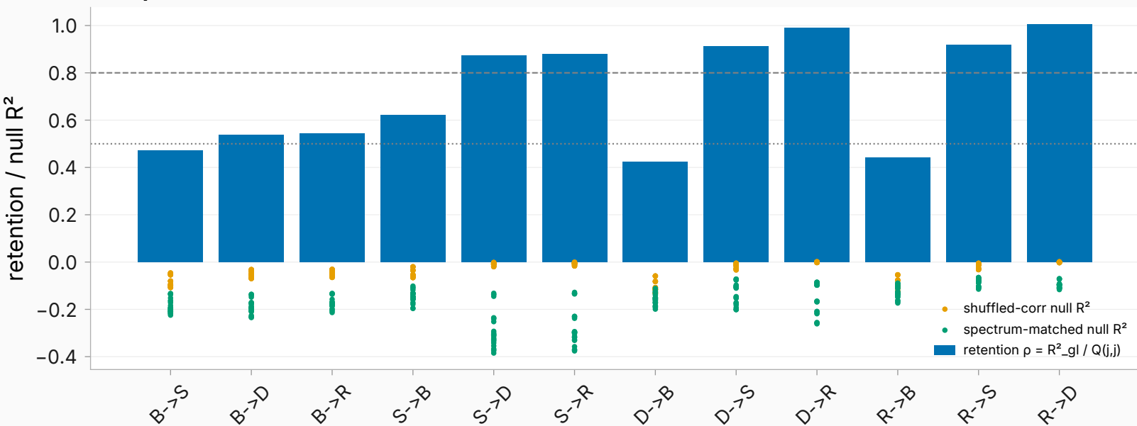
Per-pair retention with matched nulls (0.8 conf / 0.5 kill bars)
