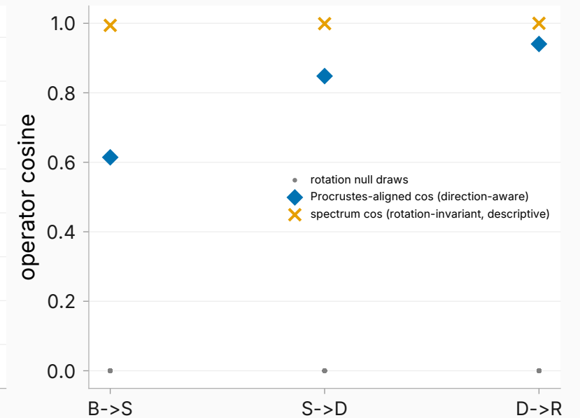
Direction-aware vs spectrum-only cosine
