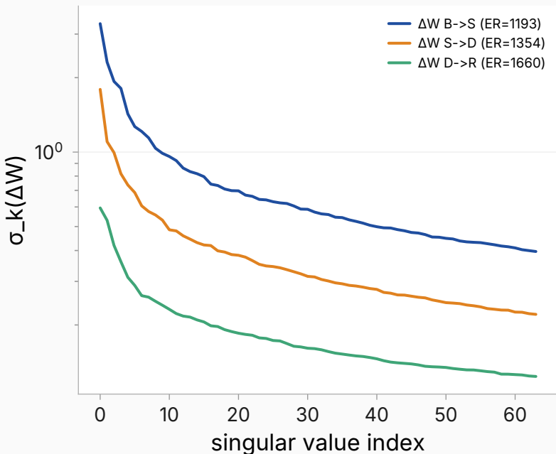
\Delta W spectra (top 64)
