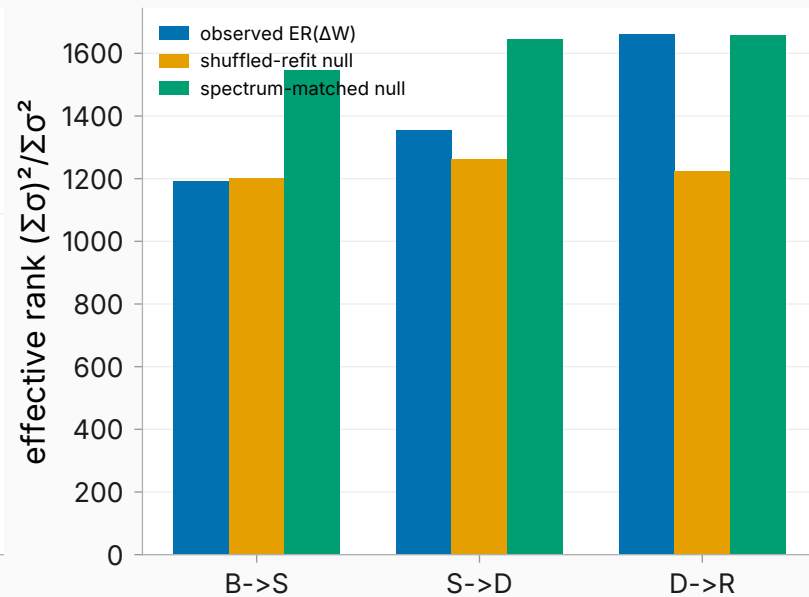
ER( \Delta W ) vs matched nulls
