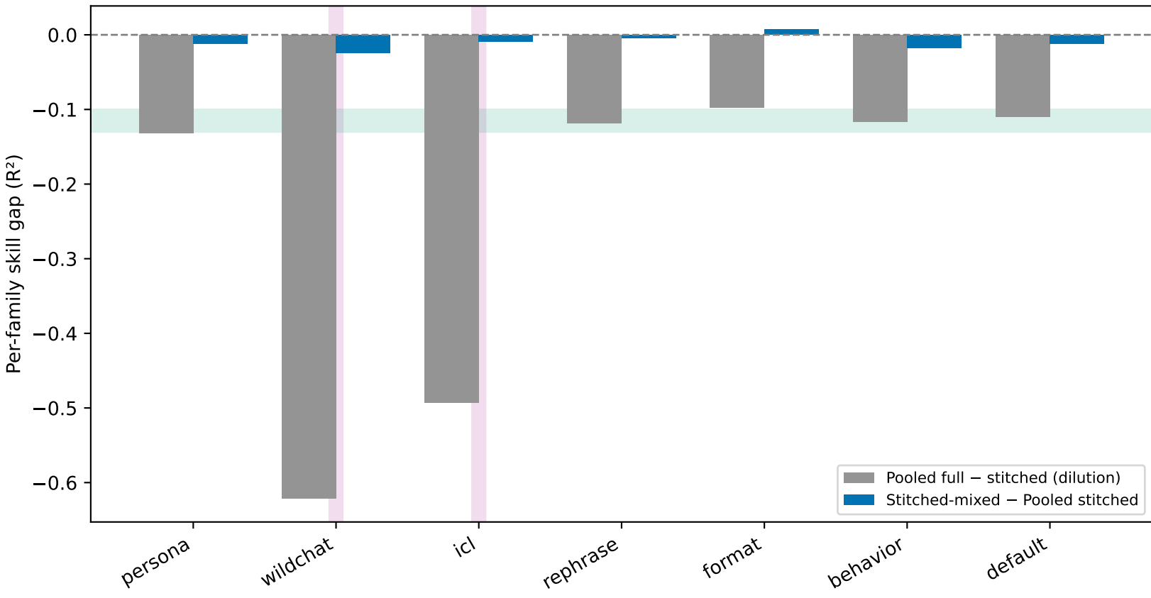
Dilution mechanism — UC held-out families, L18
