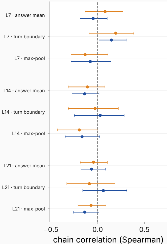
harmful-compliance (EM)
