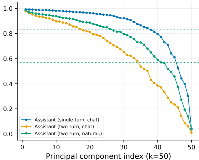
Output-subspace alignment (layer 19)
