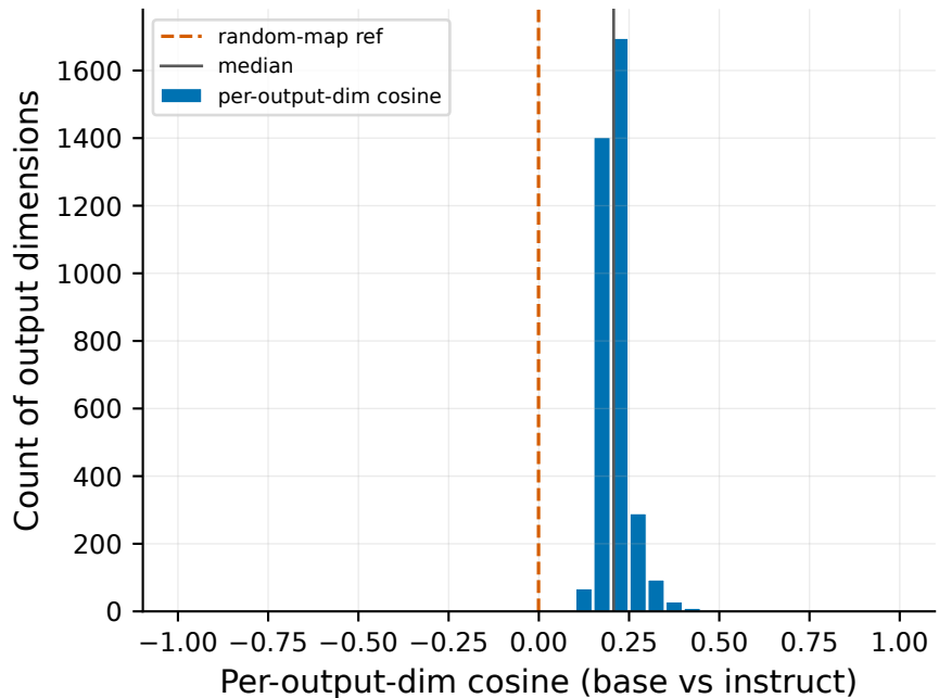
Map coefficient agreement (Assistant (single-turn, chat), layer 19)
