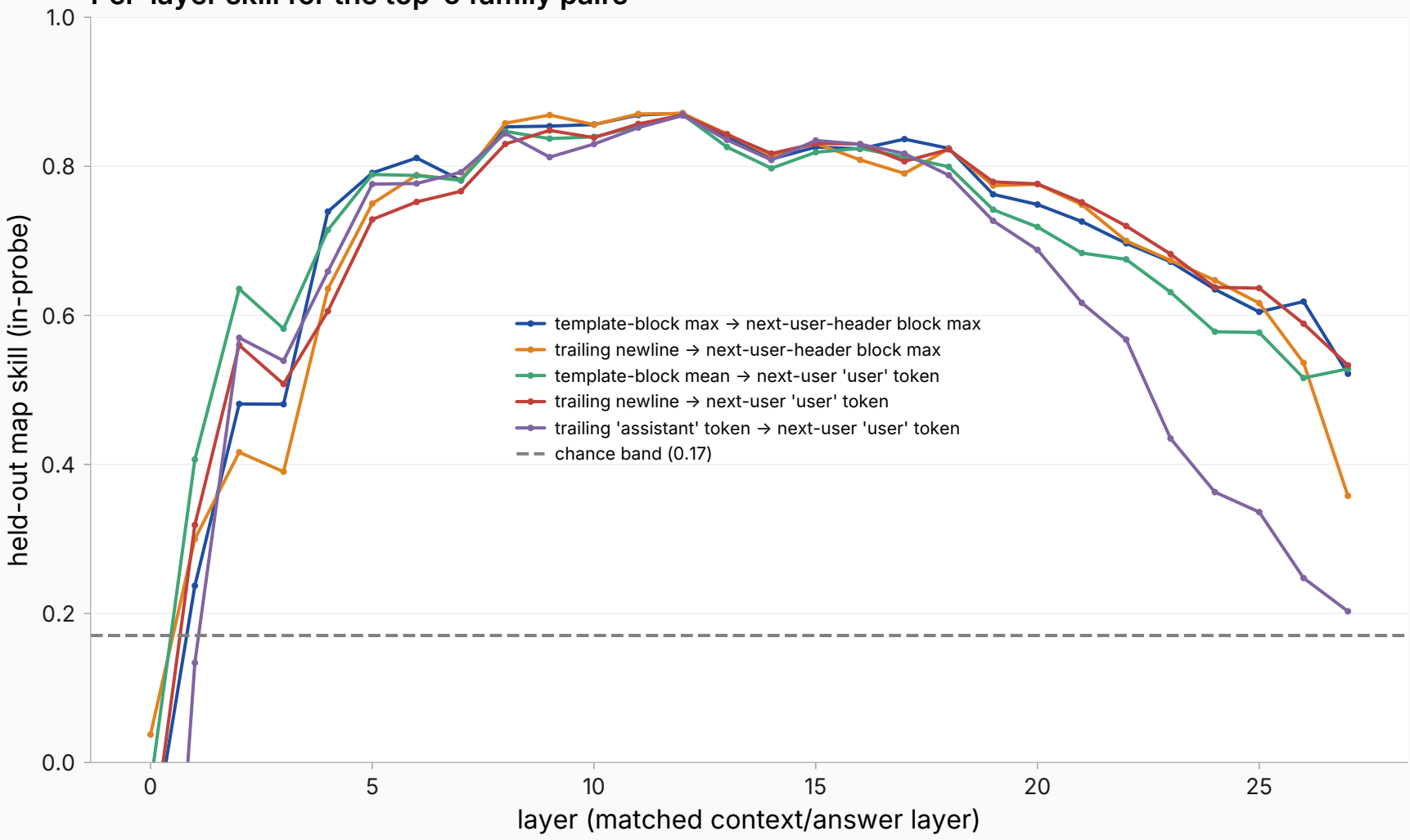
Per-layer skill for the top-5 family pairs
