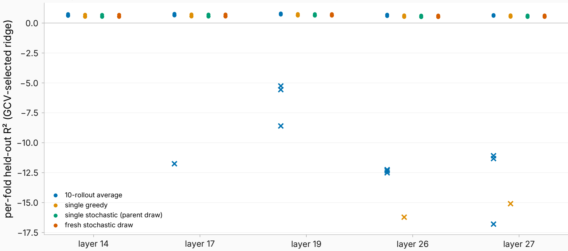
GCV per-fold fits: circles = healthy \lambda ( \geq 316 ), crosses = grid-floor \lambda ( \leq 0.032 )
