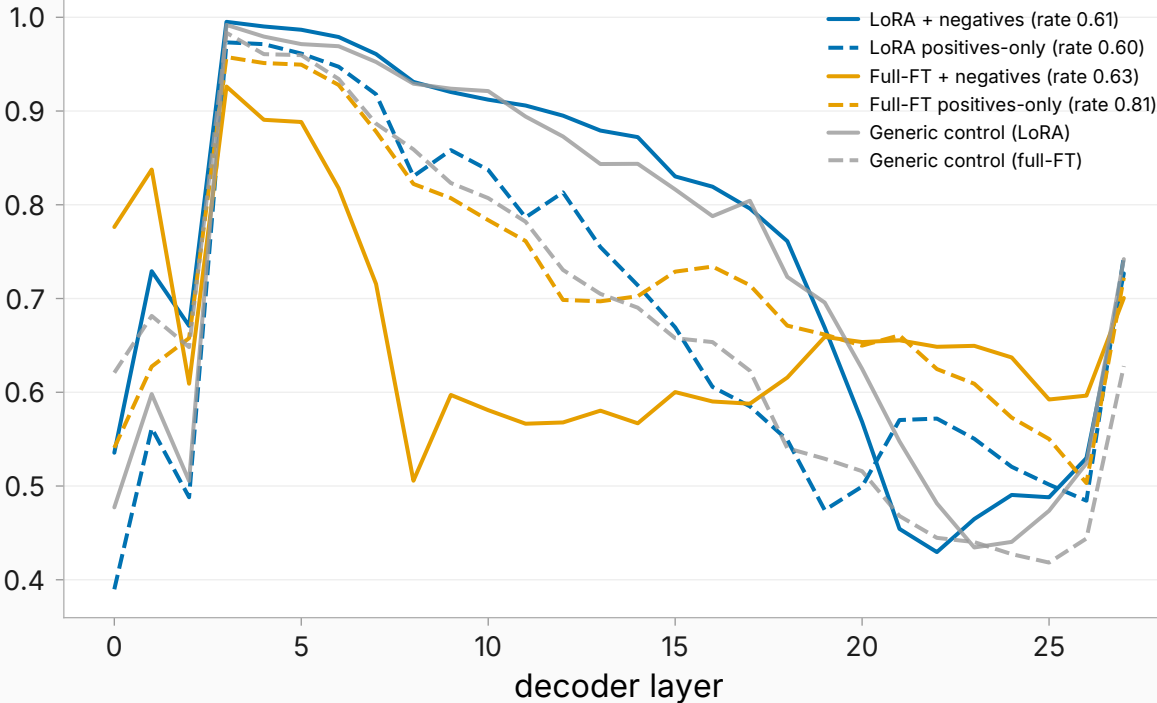
sycophancy activation shift — prefix arm (selected checkpoint)
