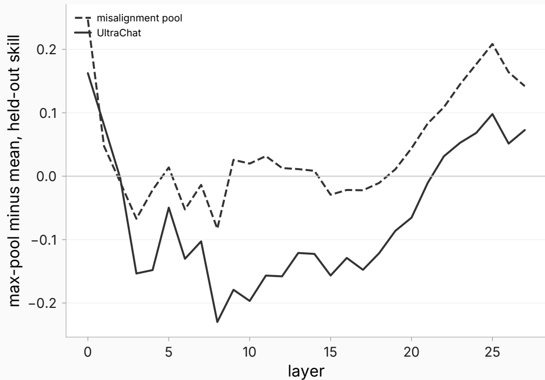
The late-layer max-pool edge shrinks on UltraChat
