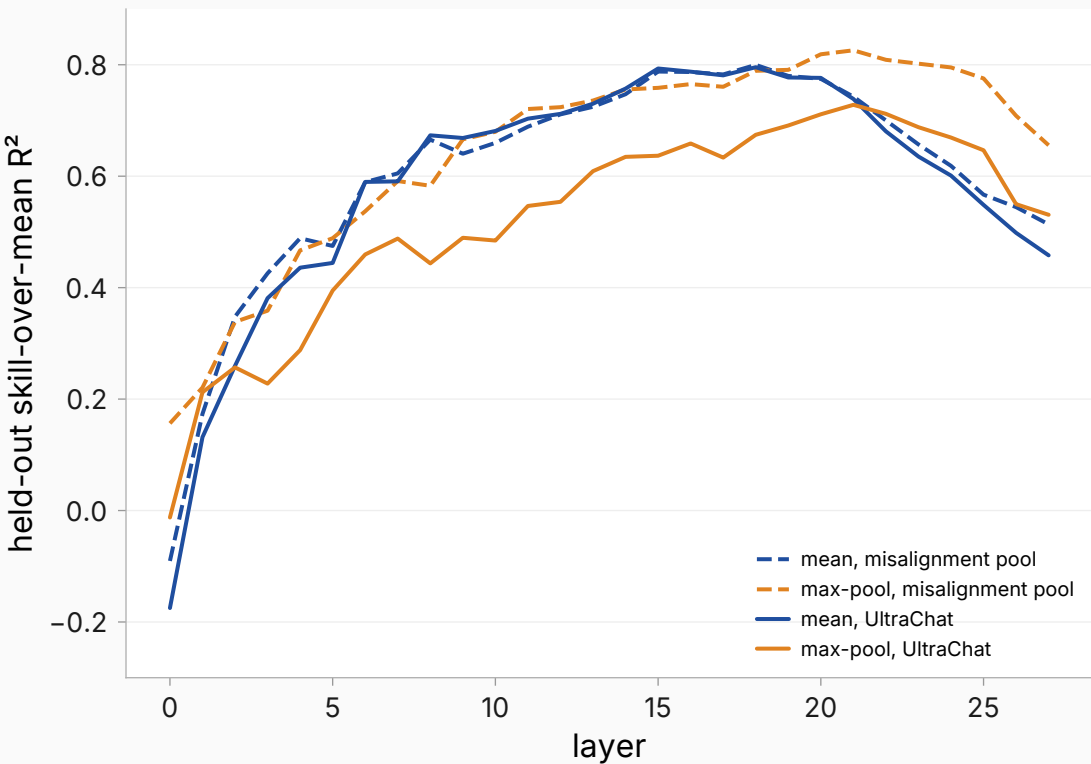
Mean transfers across genres; max-pool drops on UltraChat
