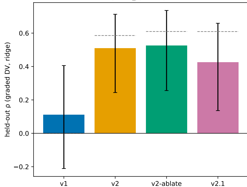
headline p + \sqrt{r_{yy}} ceilings (dashes)
