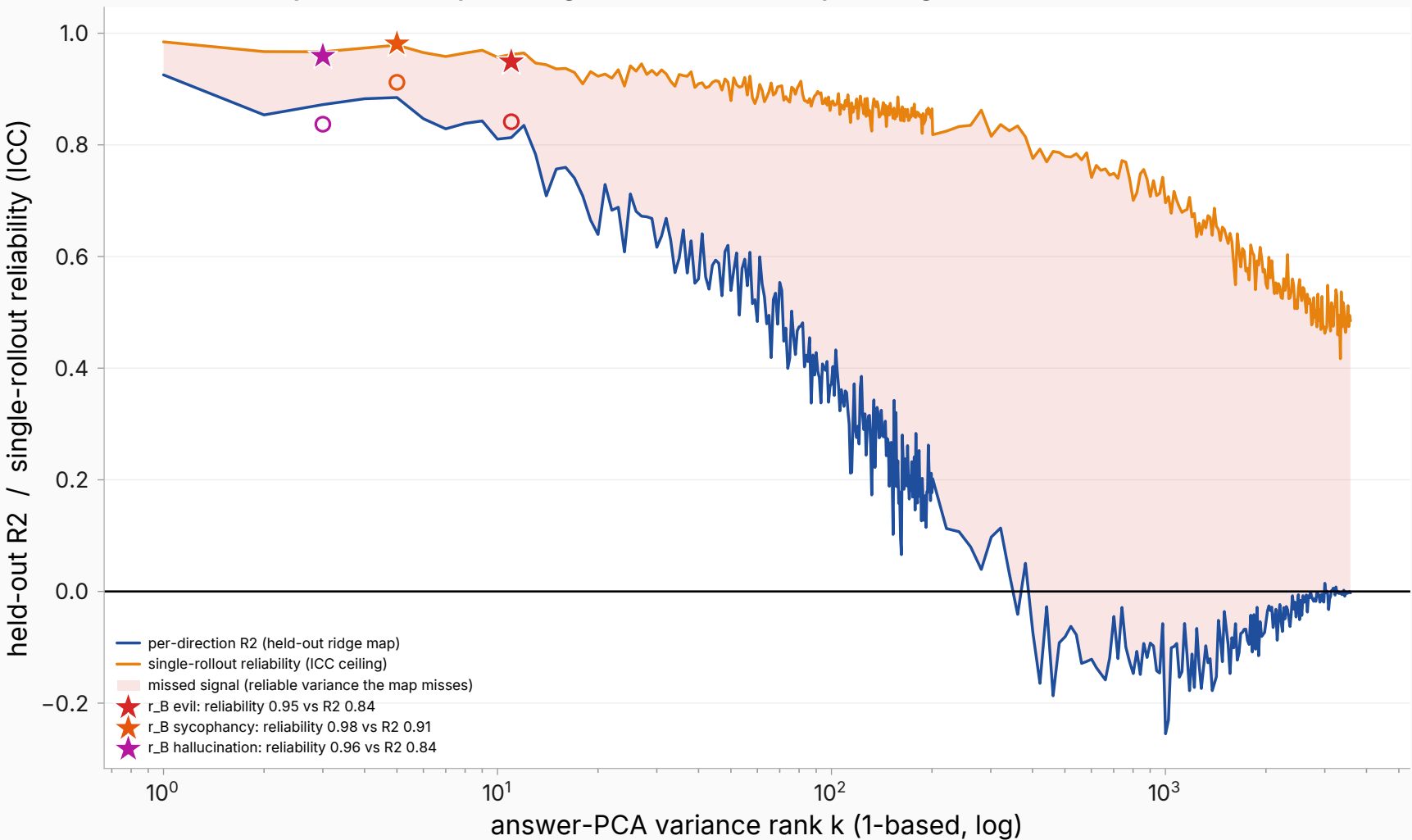
Per-direction predictability vs single-rollout reliability ceiling at L19
