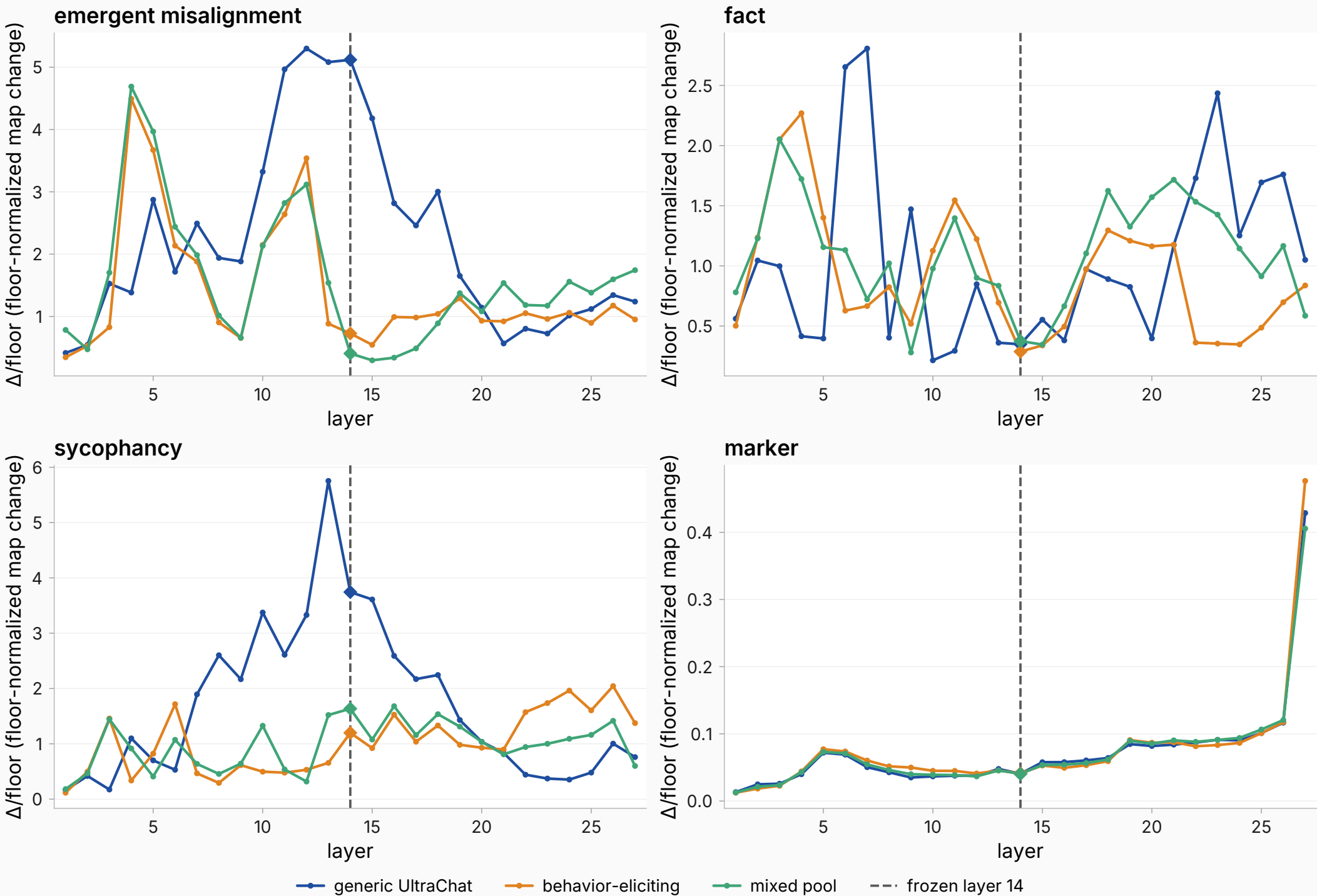
Per-layer floor-normalized map change (M0 vs M + ), by behavior × query pool — frozen layer 14 marked
