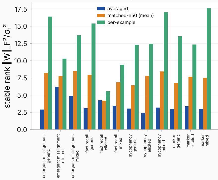
stable rank (trained arm, \lambda=1e3 )
