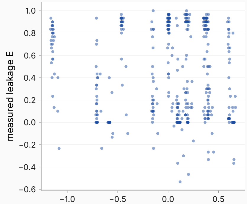
trained map, layer 21: Spearman -0.09 (n=480)
