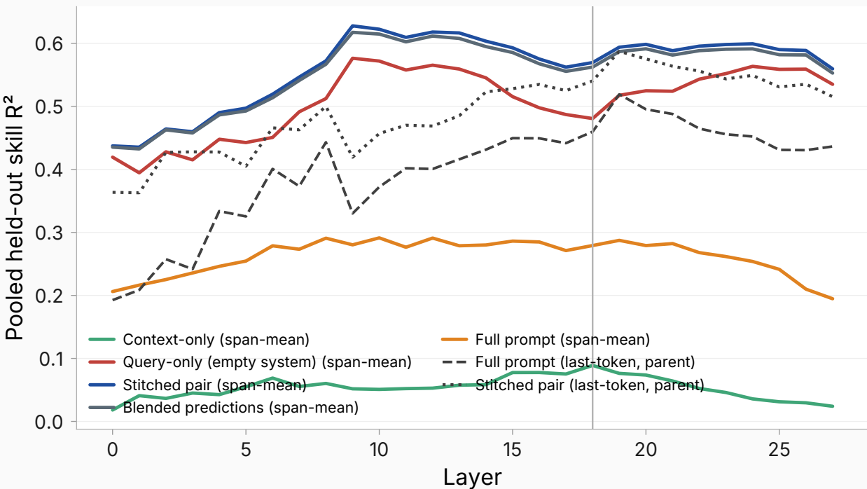
Skill by layer under the span-mean summary, UltraChat grid
