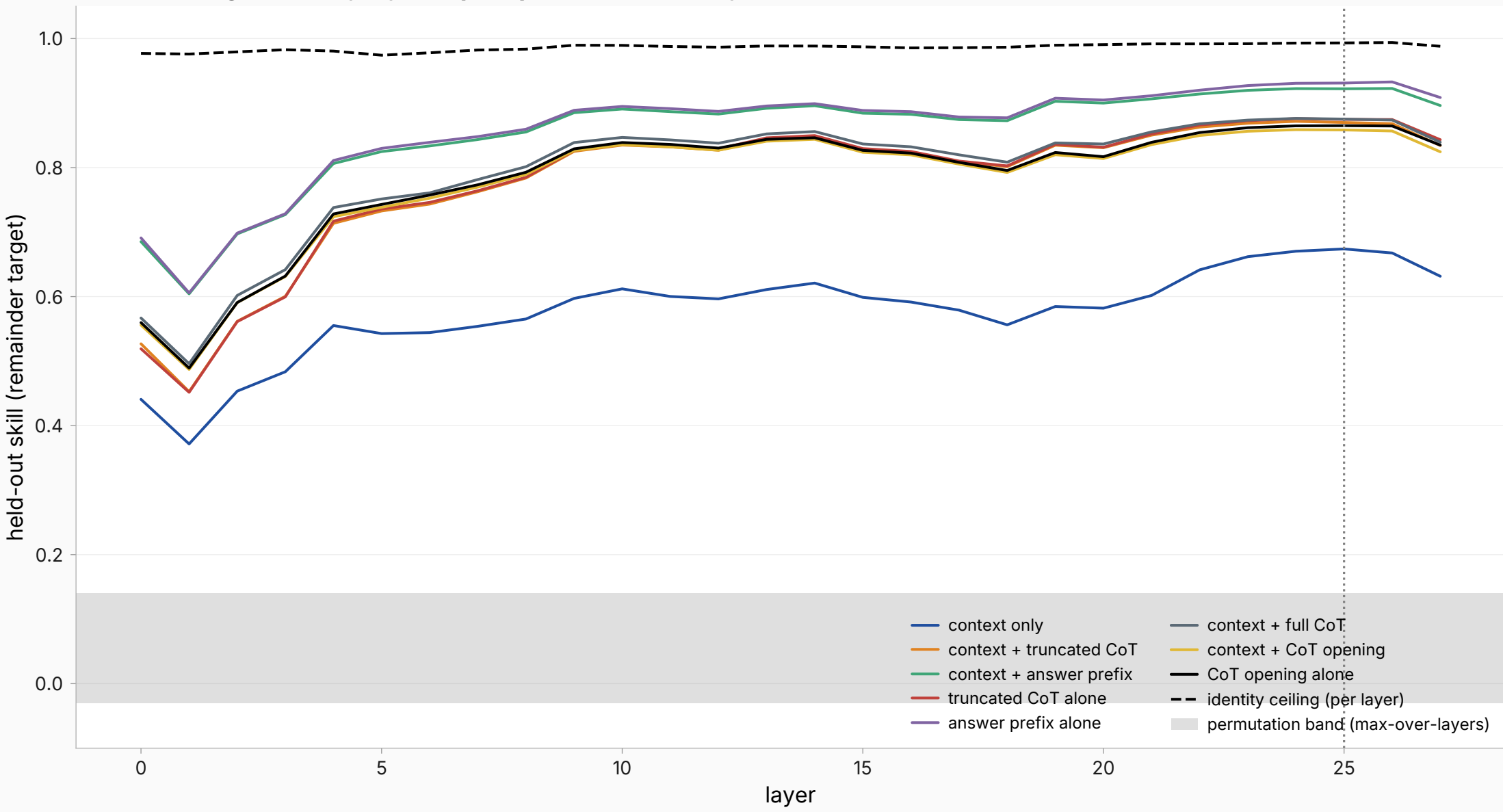
matched-length arms by layer — per-question (frozen layer 25 dotted)
