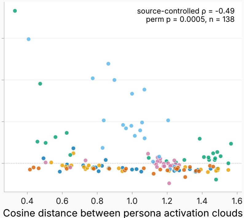
Runner-up: cosine, layer 2 (end of system prompt)
