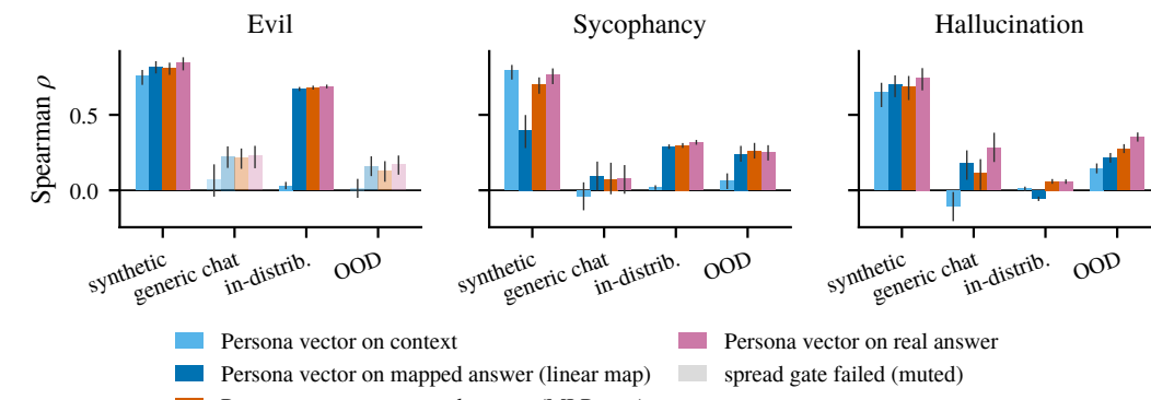
Figure 9. Spearman \rho between a persona-vector readout and the judged behavior, per regime. Bars: readout on the context , on the map-predicted answer (linear, MLP), and on the real answer an oracle, it needs the answer generated. Muted bars failed the spread gate.
