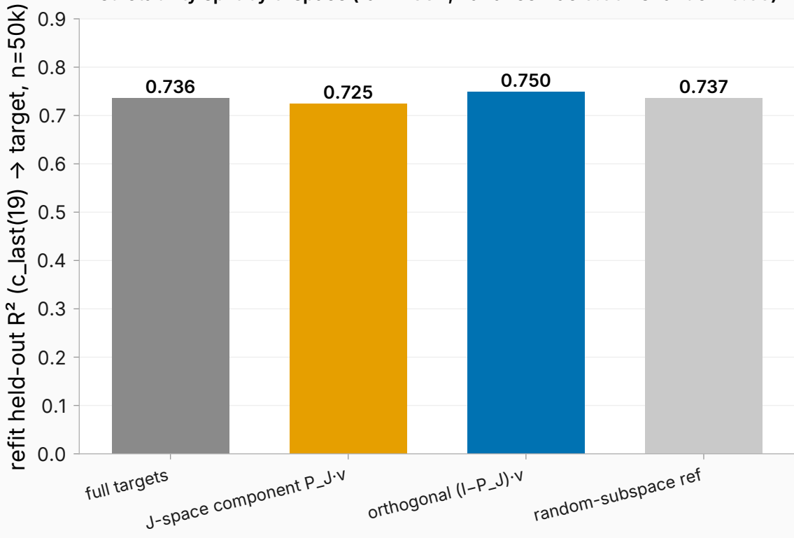
Predictability split by J-space (rank 1884; variance frac 0.56 vs random 0.53)
