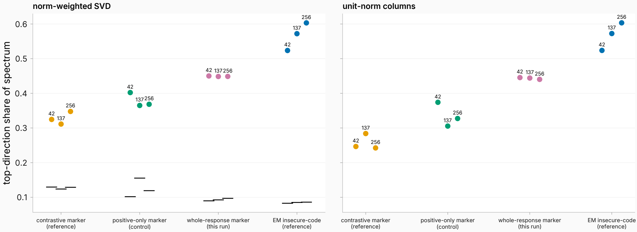
Trained-model-text shift-spectrum concentration by training condition (ticks = per-cell sign-flip null p95)
