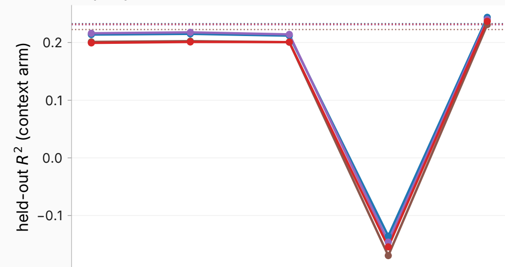
on-policy — instruct
