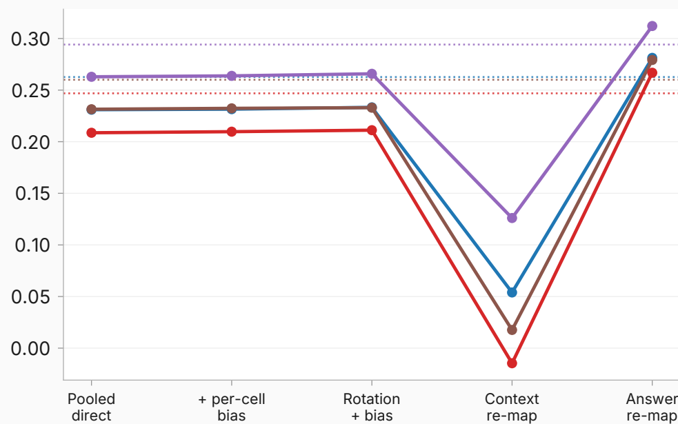
inserted — base
