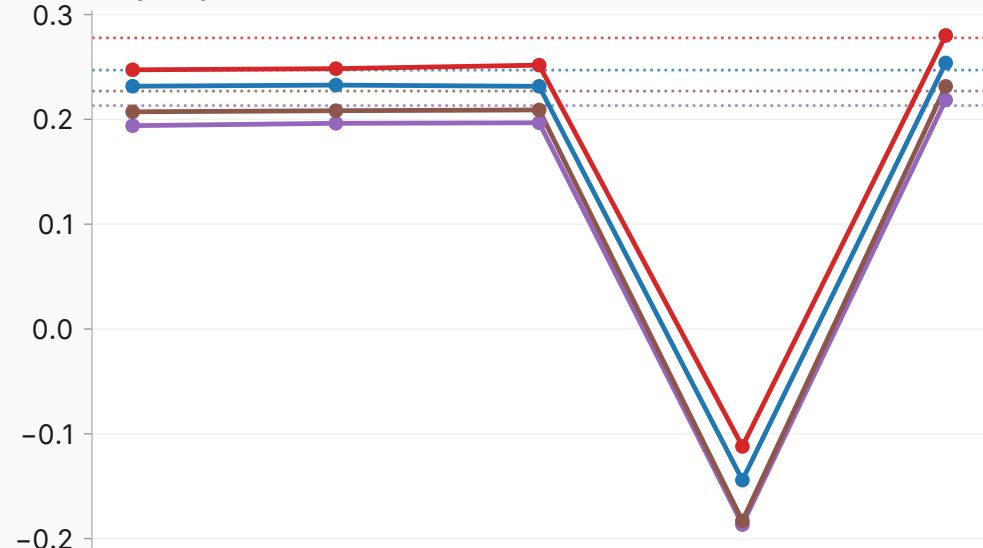
on-policy — base
