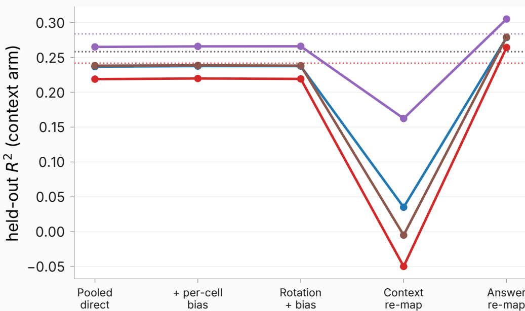
inserted — instruct
