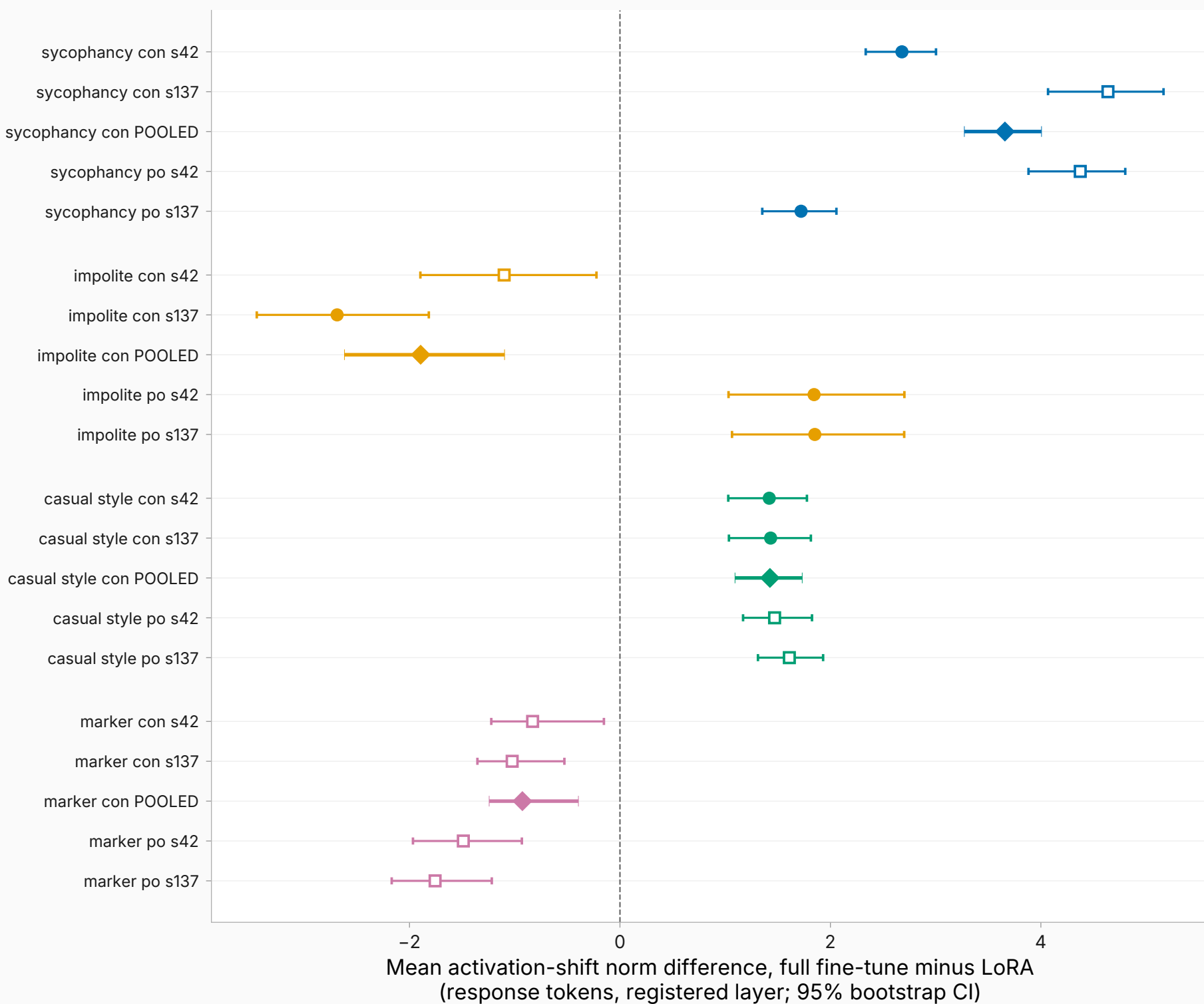
Full fine-tuning shifts activations farther for sycophancy and casual style, less far for impolite (con) and the under-dosed marker — filled = dose-matched pair
