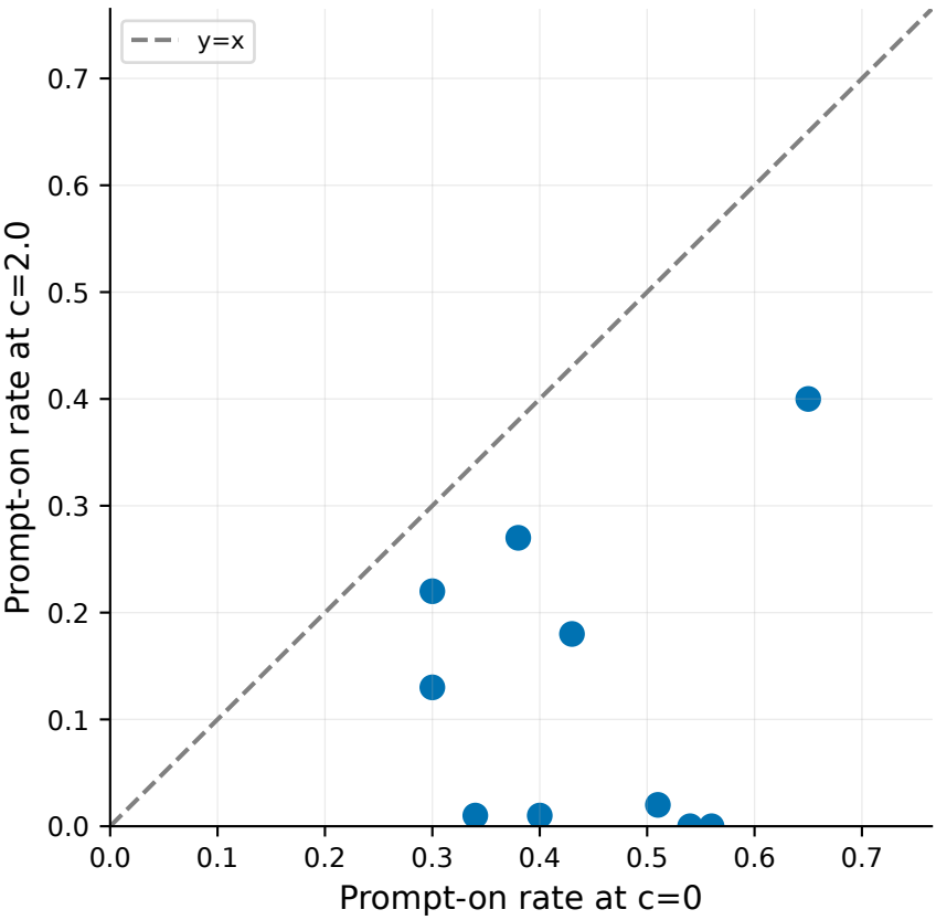
Sign-check: 10/10 personas below diagonal
