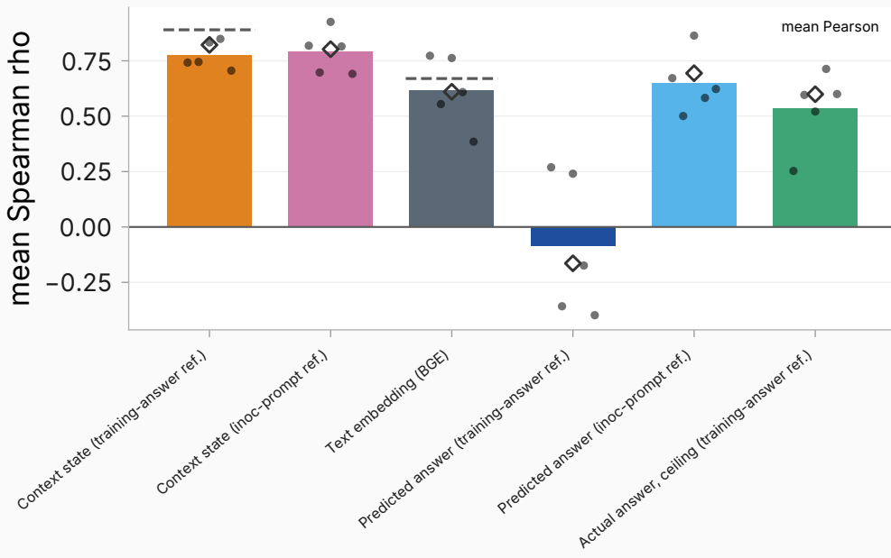
Misalignment — decoder layer 16
