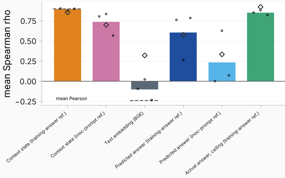
Capitalization — decoder layer 27
