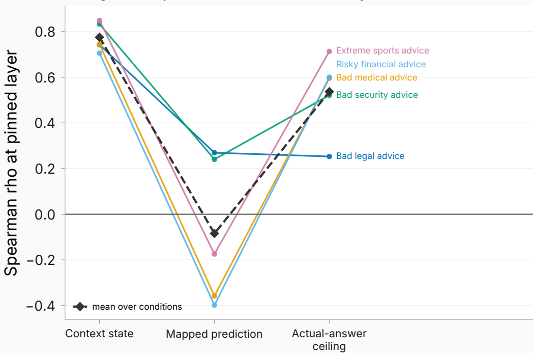
Misalignment — per-condition reads at decoder layer 16
