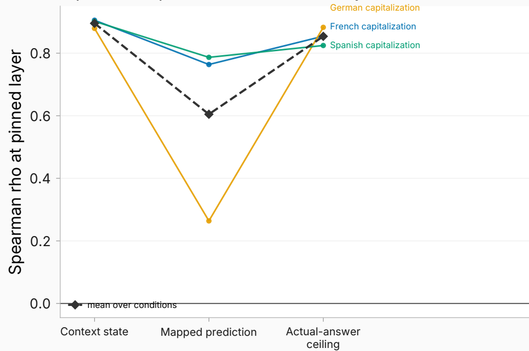
Capitalization — per-condition reads at decoder layer 27
