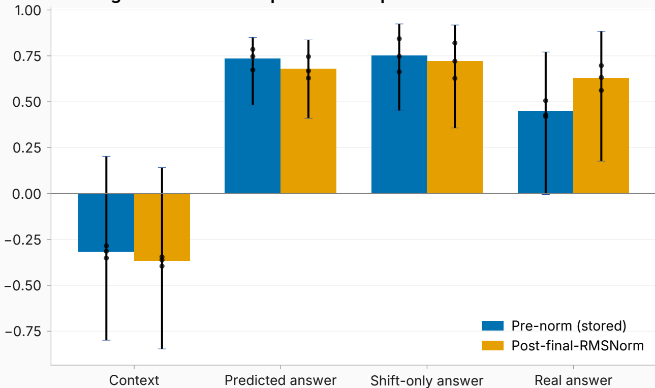
Training-reference arms: pre-norm vs post-final-RMSNorm
