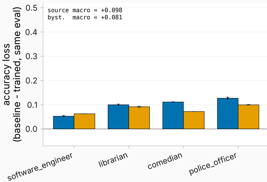
(C) generic-CoT train -> generic-CoT eval matched-scaffold control
