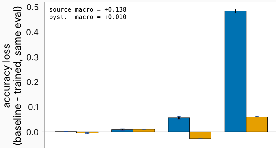
(C) generic-CoT train -> generic-CoT eval matched-scaffold control
