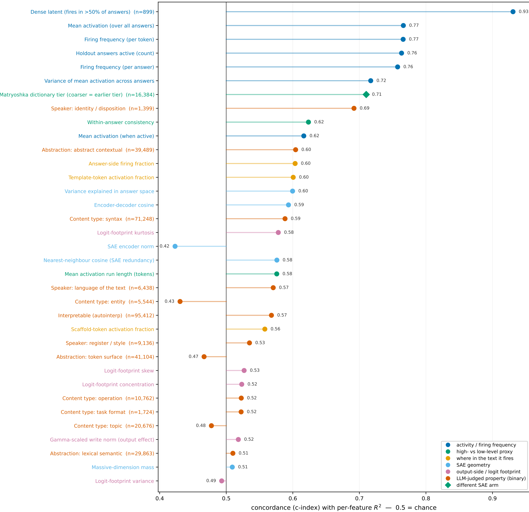
Which feature properties predict how well the context→answer map predicts a feature? concordance over all pairs · sorted by predictive power |c - 0.5| \cdot n = 120,716 features
