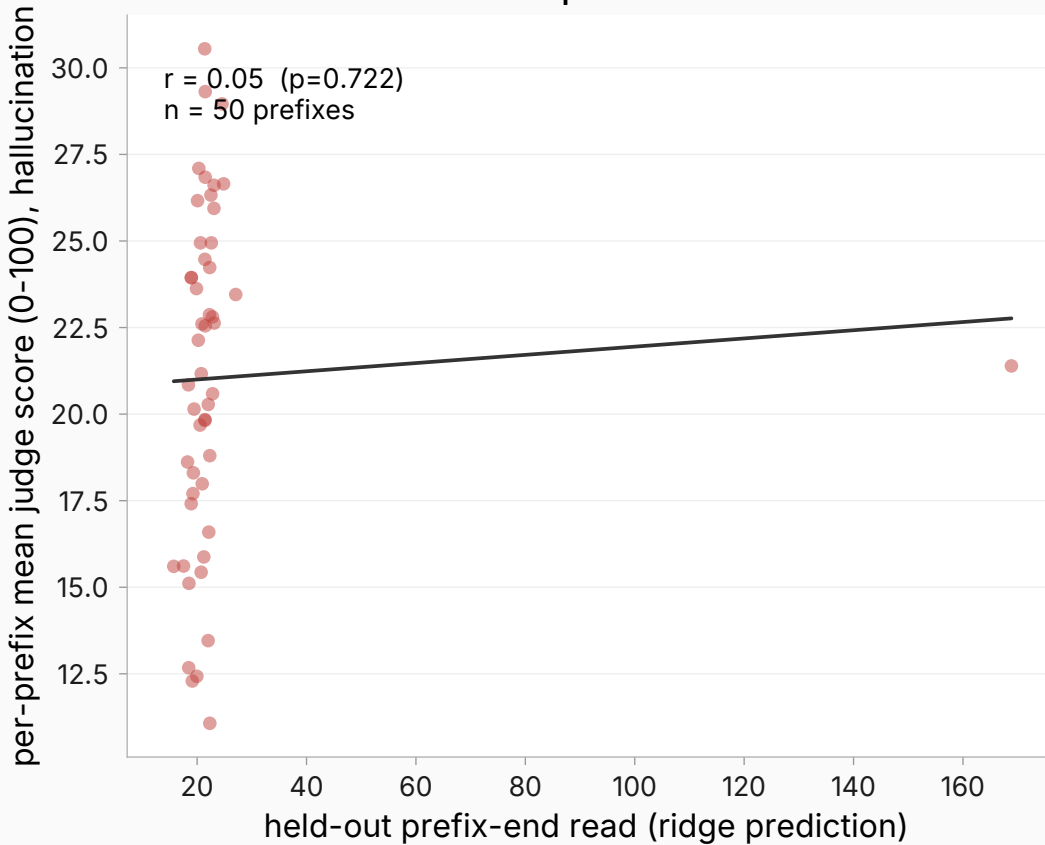
Base model — hallucination — prefix-end
