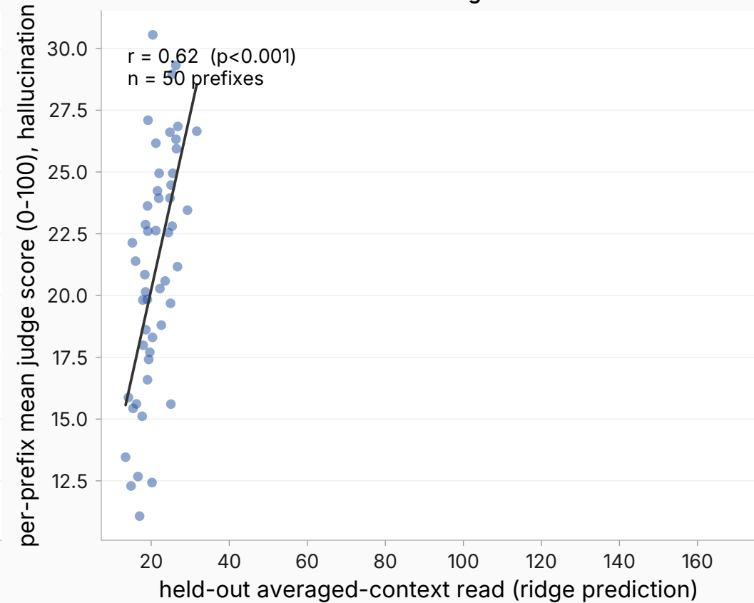
Base model — hallucination — averaged-context
