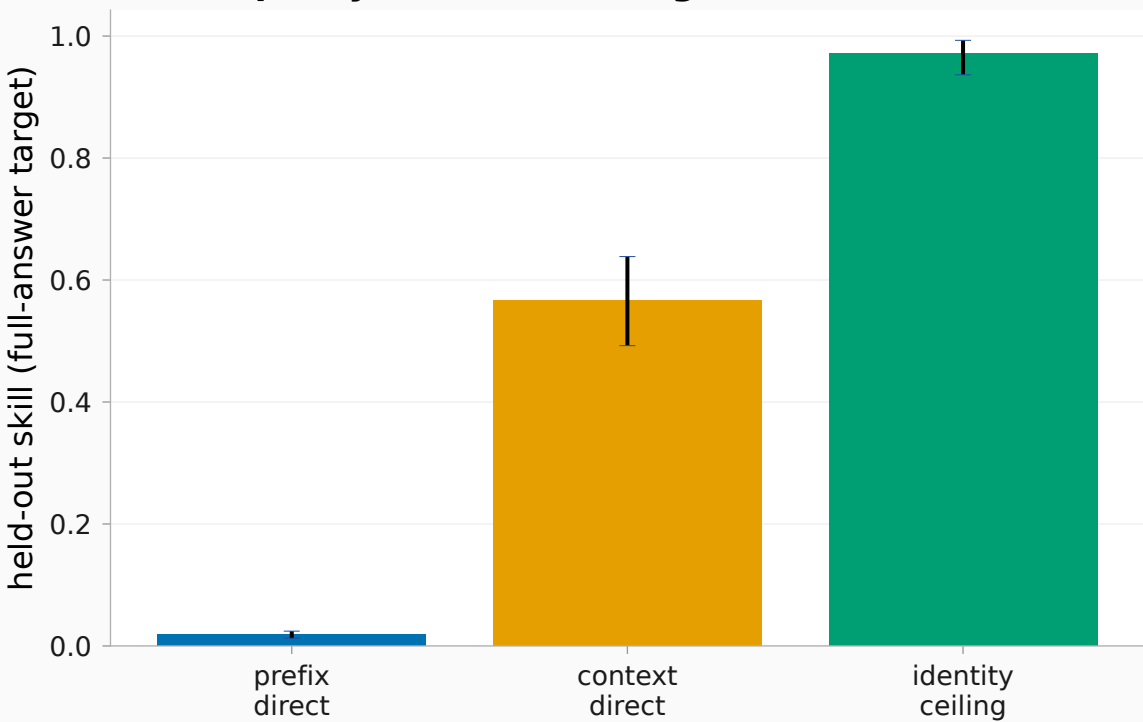
Parent-parity full-answer target @ L24 (indiv)
