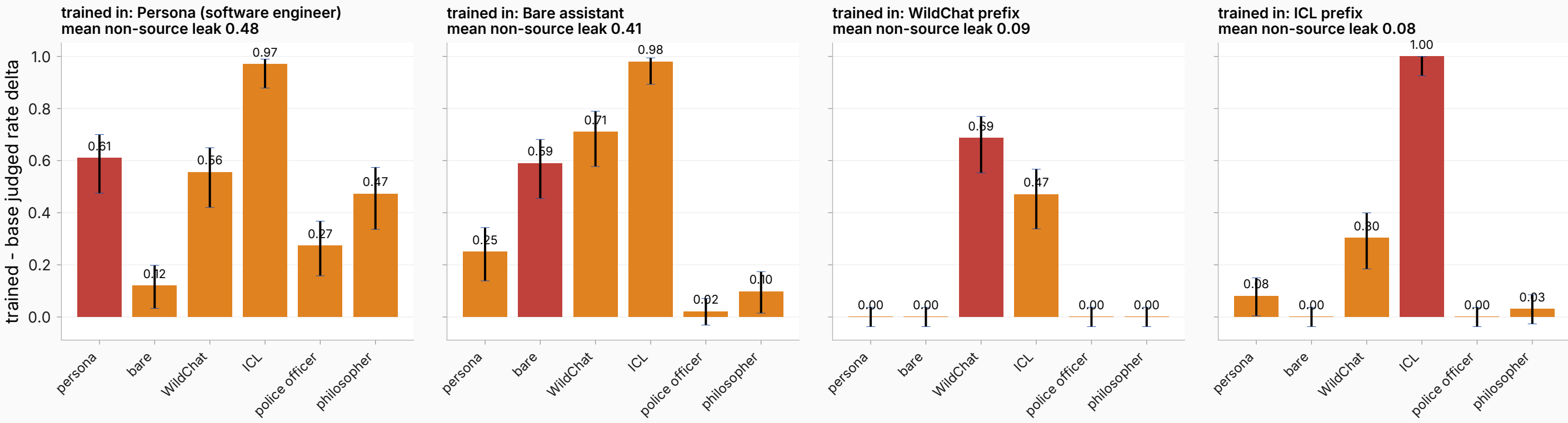
Leakage panel at the four verdict arms (dark red = training/source context; orange = bystander contexts; n=100 per cell)
