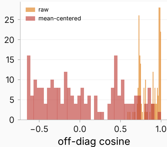
issue406_gram_L21 (approx)
