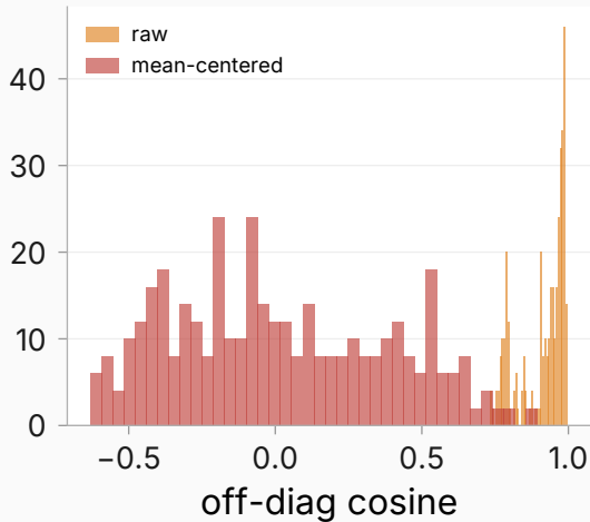
extraction_method_a_L20
