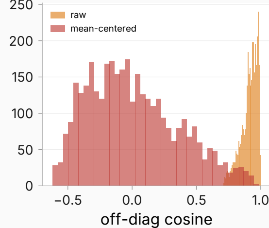
issue505_pv_L21
