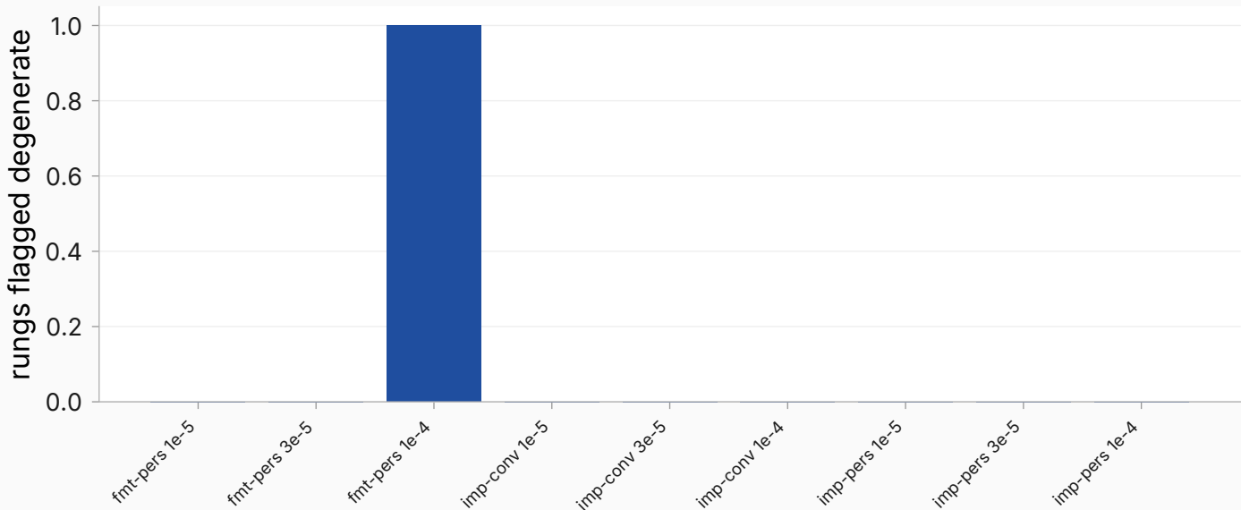
degenerate-output guard flags per run (length/4-gram; flag-only)
