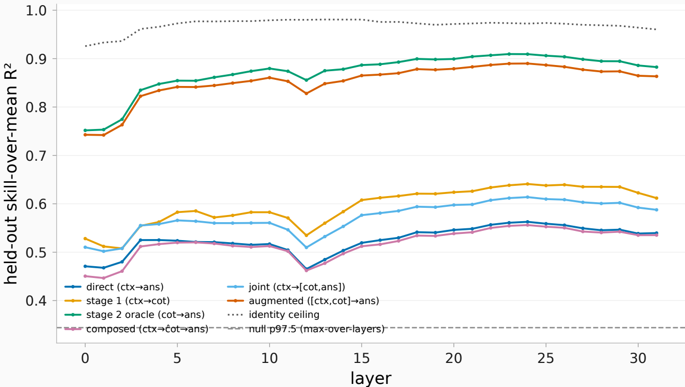
CoT-decomposition arms — indiv, mean/mean, LOCO
