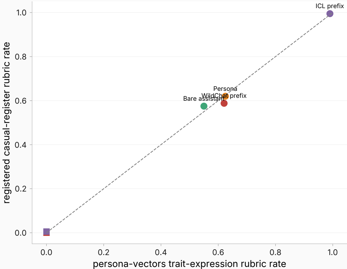
Instrument parity on the same Tier-2 completions (circles = trained verdict arms, squares = base arms; max gap 0.033)
