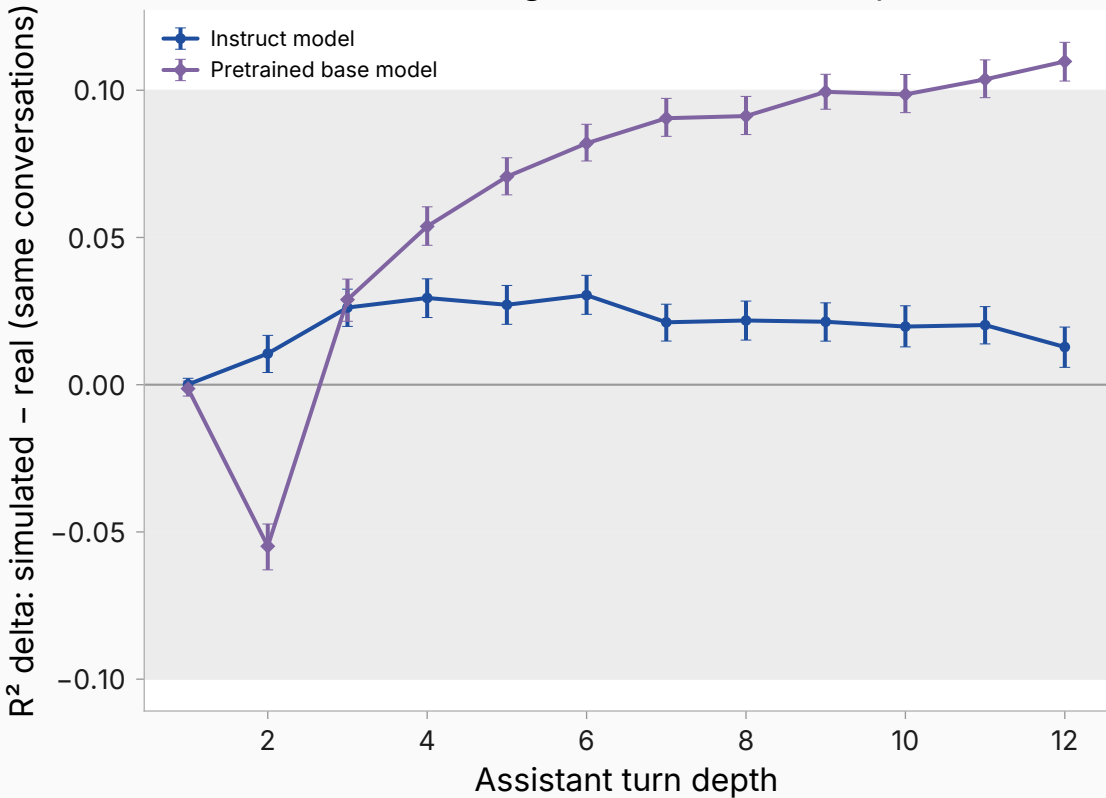
Simulated-vs-real bridge (seed intersection, \pm 0.10 band)
