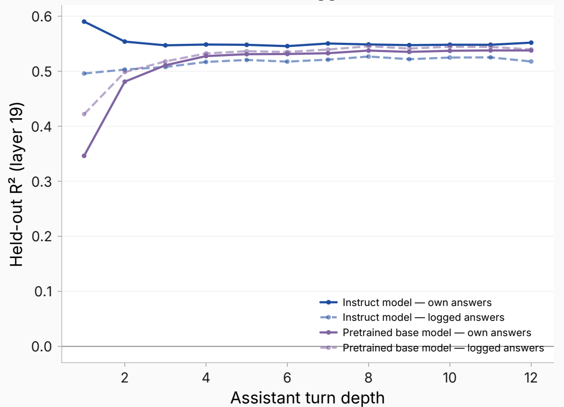
Real conversations: own vs logged answers (n \approx 5000/turn)
