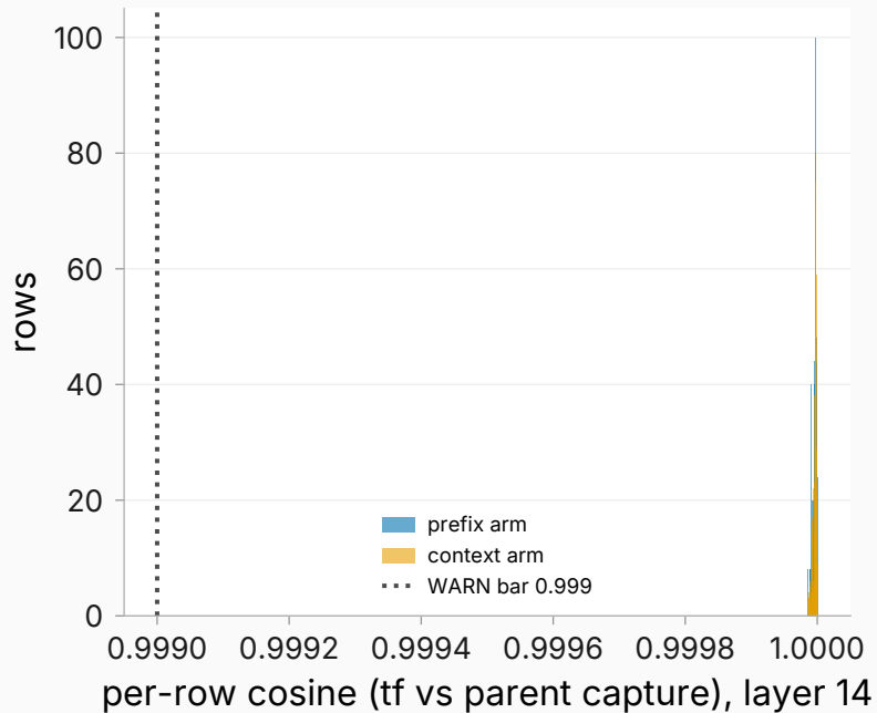
prefix/context parity check — same prompt tokens across capture rounds
