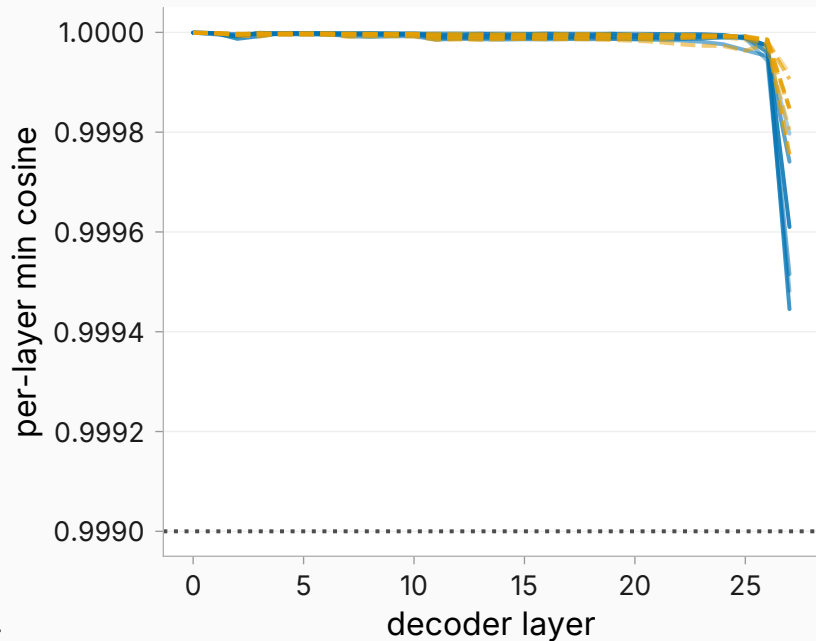
prefix/context parity check — same prompt tokens across capture rounds
