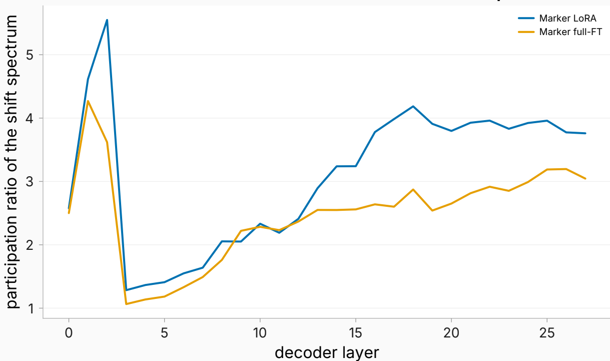
marker activation shift — context arm (selected checkpoint)
