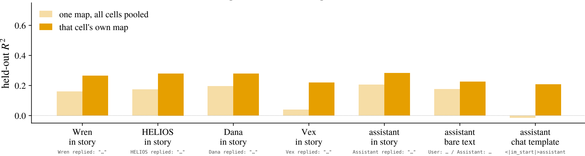
Pooled vs cell-specific fit, evaluated per cell — Qwen-2.5-7B (base)
